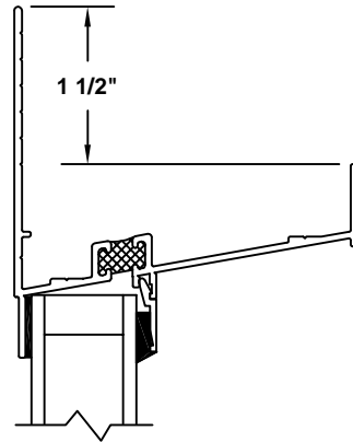
FLANGED HEAD
