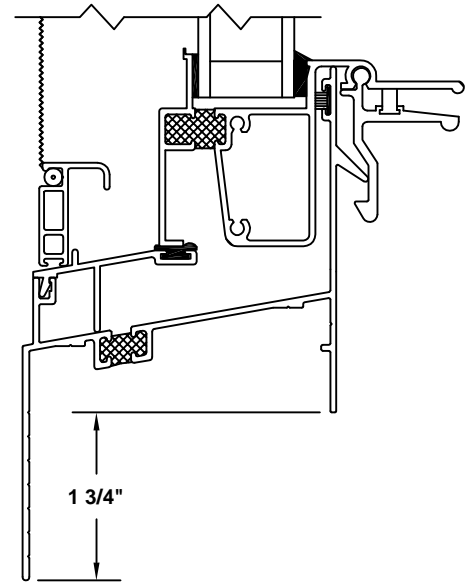
FLANGED SILL
