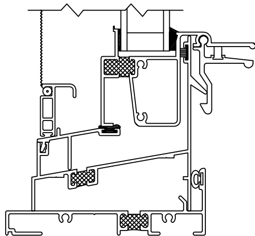
#8126 STARTER SILL
