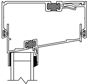
#8124-RECEPTOR #8125-CLIP
