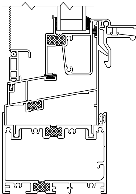
#8131/#8132 10# SUBSILL/STIFFENER
