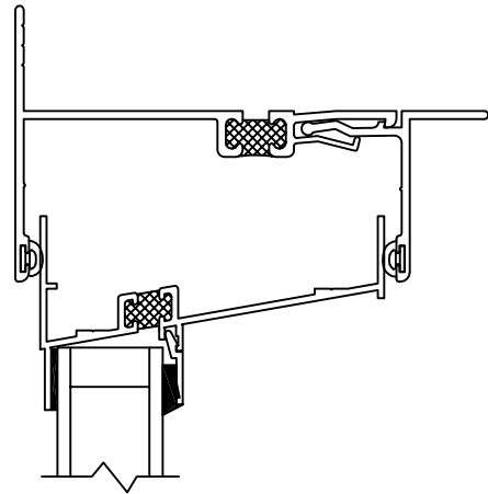
#8127-RECEPTOR W/FLANGE #8128-CLIP W/FLANGE
