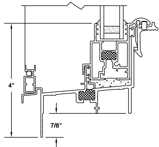
FLANGED SILL
