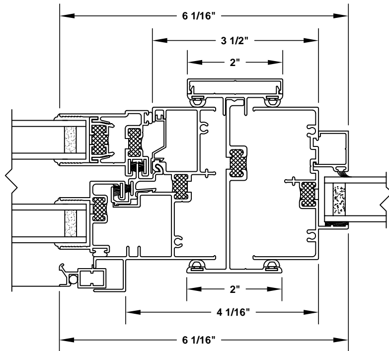
3-PCS MULLION
