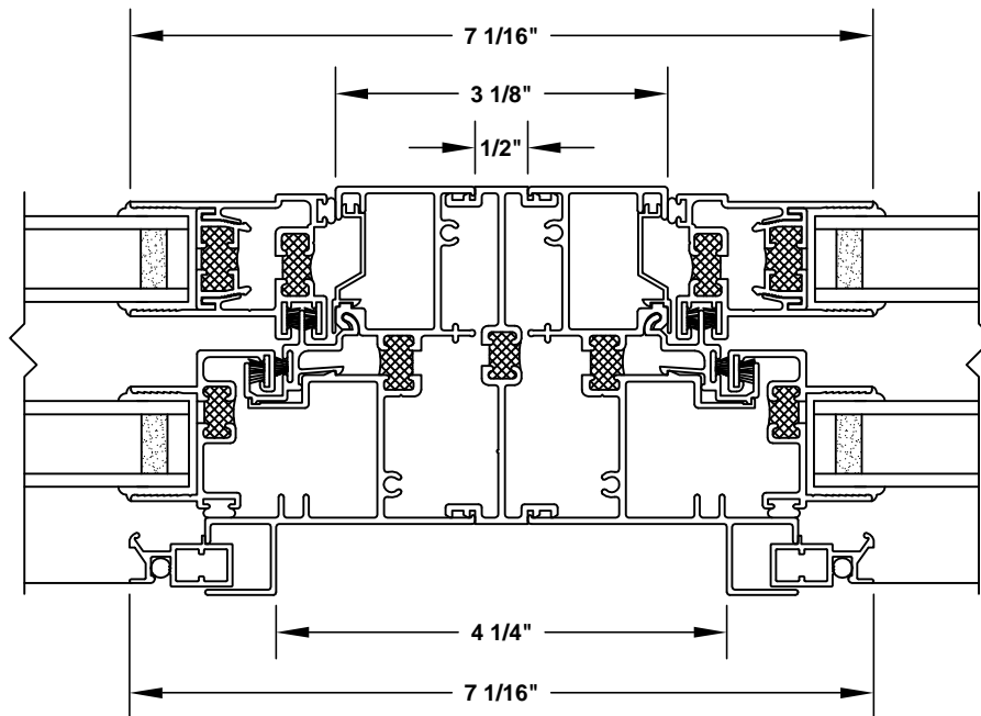
THERMAL STACK MULLION
