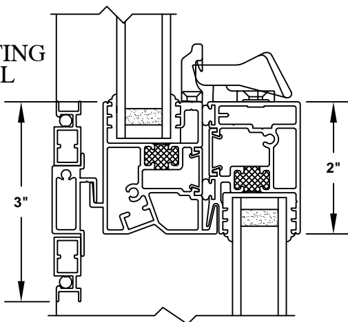
③ SILL
